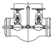
With equalizing pipe and bypass valves
