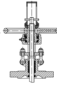
Position indicator
