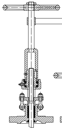
Extended stem
